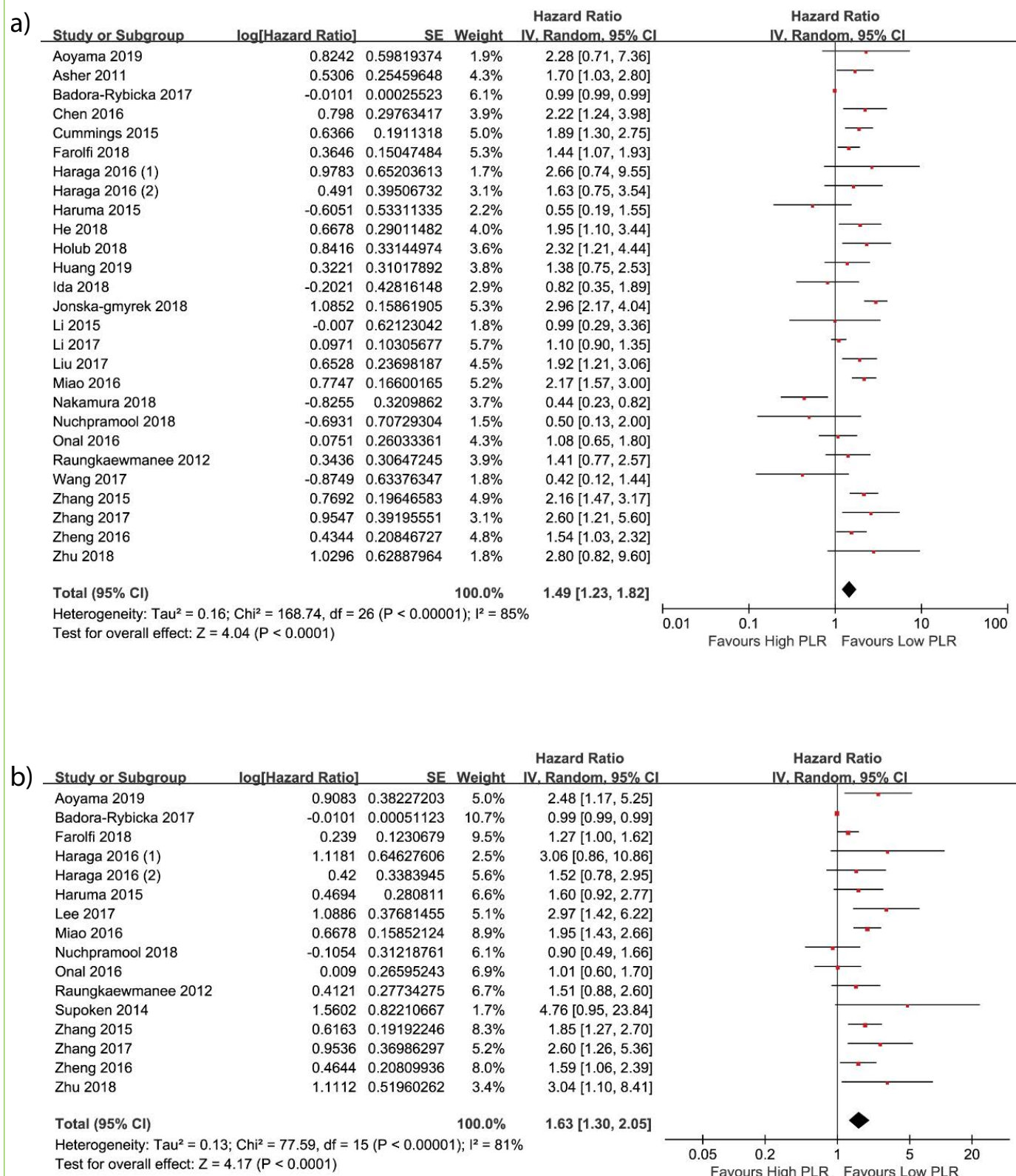
Figure 2: Forest plots showing hazard ratio for overall survival (A) and progression-free survival (B) in all studies for platelet-to-lymphocyte ratio greater or less than the cut-off. Hazard ratio for each study are represented by the squares, the size of the square represents the weight of the study in the meta-analysis, and the horizontal line crossing the square represents the 95% confidence interval (CI). All statistical tests were two-sided.
