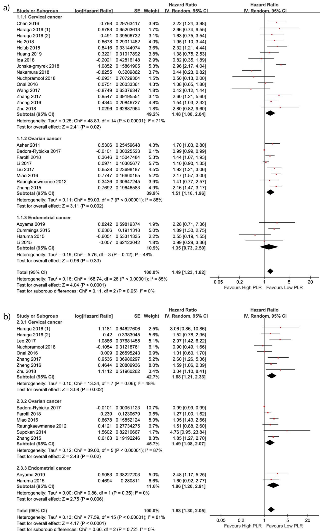
Figure 3: Forest plots showing hazard ratio for overall survival (A) and progression-free survival (B) by primary tumor for platelet-to-lymphocyte ratio greater or less than the cut-off. Hazard ratio for each study are represented by the squares, the size of the square represents the weight of the study in the meta-analysis, and the horizontal line crossing the square represents the 95% confidence interval (CI). All statistical tests were two-sided.
