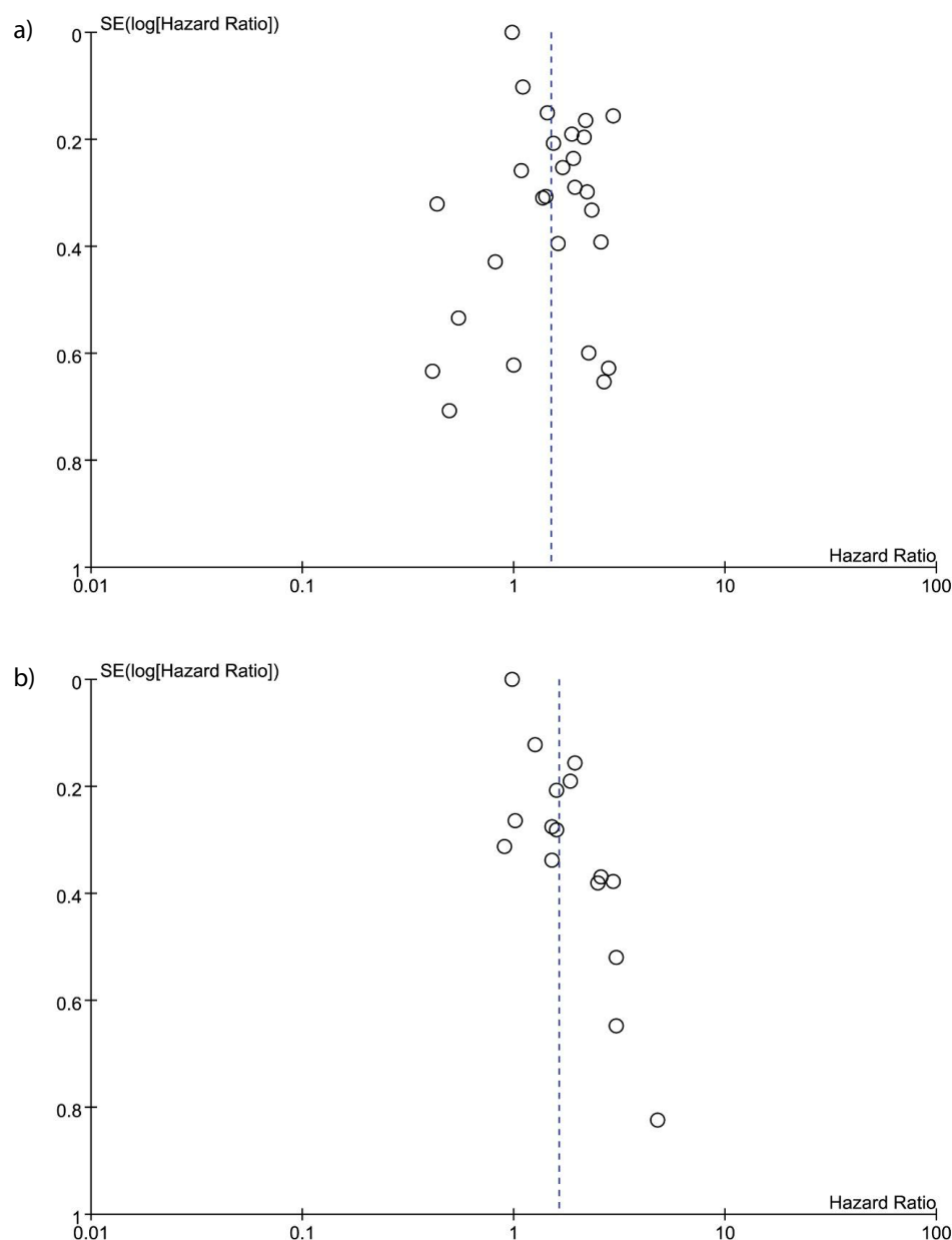
Figure 4: Funnel plot of hazard ratio for overall survival (A) and progression-free survival (B) for high platelet-to-lymphocyte ratio (horizontal axis) and the standard error (SE) for the hazard ratio (vertical axis). Each study is represented by one circle. The vertical line represents the pooled effect estimate.
