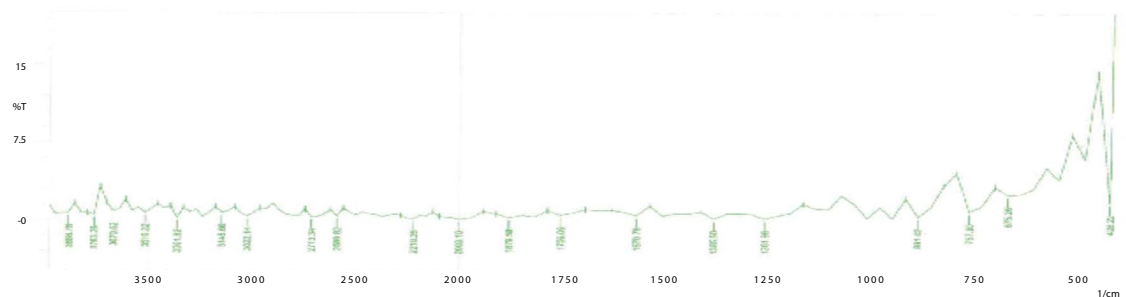
Figure 3: Fourier Transform Infrared spectroscopy of Olmesartan Medoxomil glyceryl monosterate soy lecithin, polysorbate 80, physical mixture and solid lipid nanoparticles formulation.
