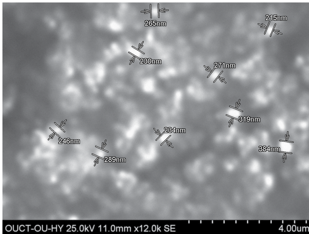
Figure 2: SEM images of BSA nanoparticles by continuous addition method.
